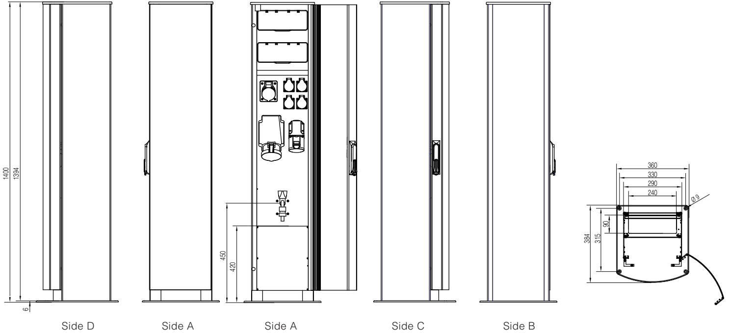
All dimensions in millimeters.
