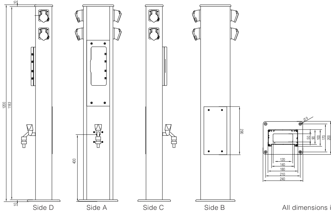
All dimensions in millimeters.
